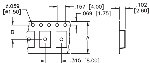
CARRIER TAPE
