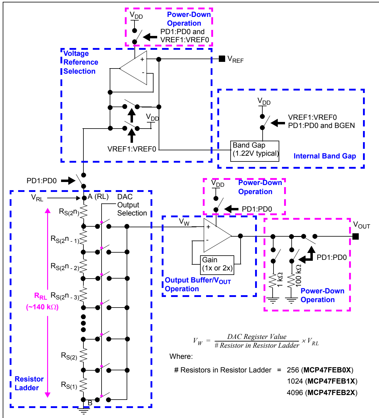
FIGURE 5-1: MCP47FEBXX DAC Module Block Diagram.
