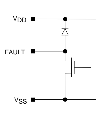
Figure 5 FAULT output block
