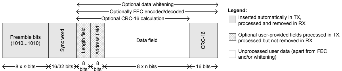
Figure 13: Packet Format
