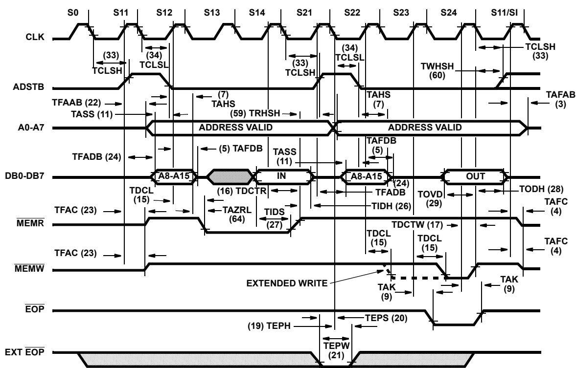
FIGURE 11. MEMORY-TO-MEMORY TRANSFER
