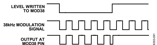
Figure 102. 38 kHz Modulation
