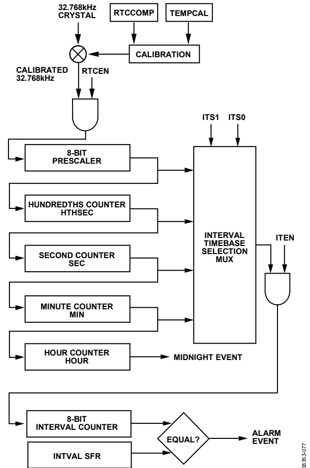
Figure 88. RTC Implementation
