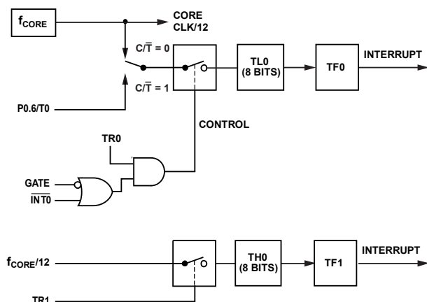
Figure 85. Timer/Counter 0, Mode 3
