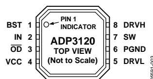
Figure 3. 8-Lead LFCSP Pin Configuration
