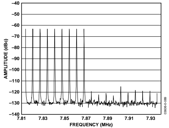
Figure 62. AD9861 Tx Path FFT, Upper-Band IMD Products of OFDM Signal in Figure 58
