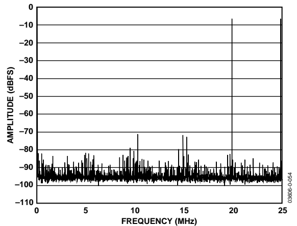
Figure 27. AD9861-80 Rx Path Dual-Tone FFT of Rx Channel A Path Digitizing 20 MHz and 25 MHz Tones
