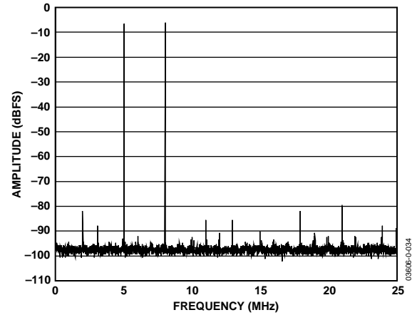
Figure 8. AD9861-50 Rx Path Dual-Tone FFT of Rx Channel A Path Digitizing 5 MHz and 8 MHz Tones
