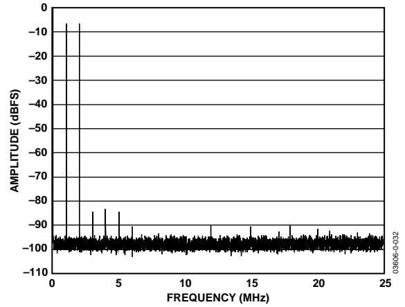
Figure 7. AD9861-50 Rx Path Dual-Tone FFT of Rx Channel A Path Digitizing 1 MHz and 2 MHz Tones
