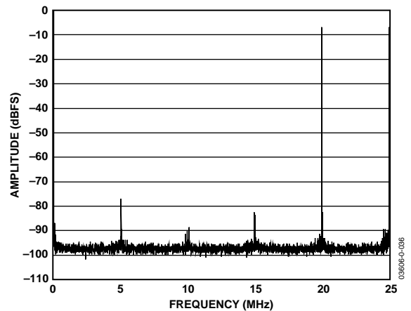
Figure 9. AD9861-50 Rx Path Dual-Tone FFT of Rx Channel A Path Digitizing 20 MHz and 25 MHz Tones
