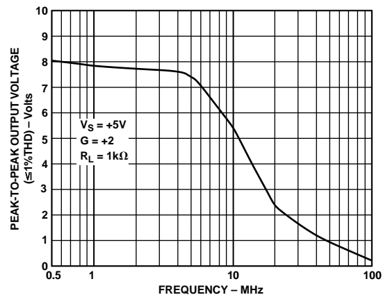
Figure 9. Output Swing vs. Frequency; V_S = \pm 5\text{ V}
