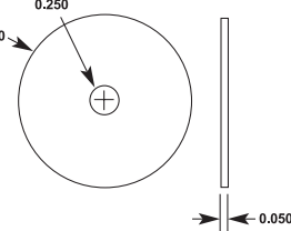
FIGURE 3. METAL COUPON
