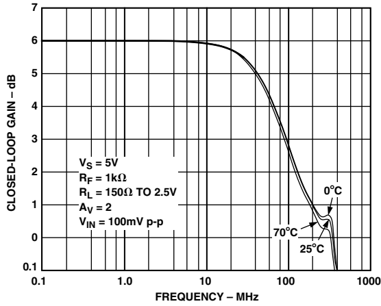
TPC 1. Frequency Response Over Temperature; V_S = 5V
