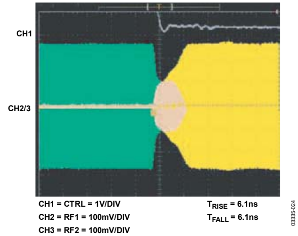
Figure 14. Switch Timing
