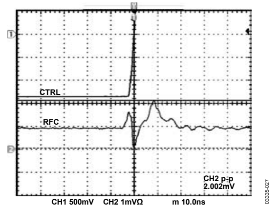
Figure 15. Video Feedthrough
